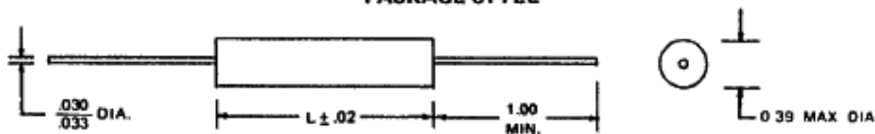
FIG. 3 PACKAGE STYLE
