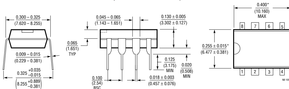
N8 Package 8-Lead PDIP (Narrow 0.300) (LTC DWG # 05-08-1510)
