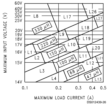
FIGURE 6. LM2594/LM2594HV-12
