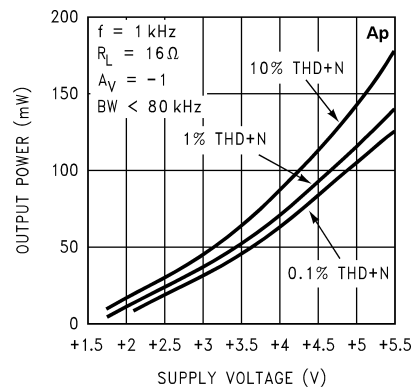
Output Power vs Power Supply
