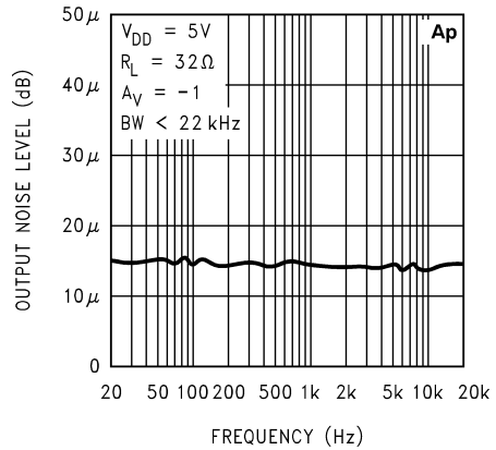
Noise Floor
