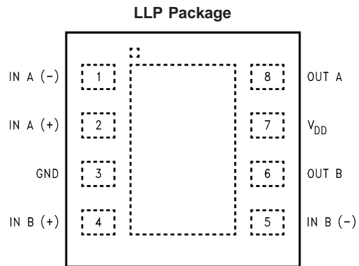
Top View Order Number HWD2108LD
