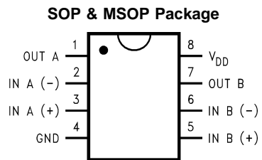
Top View Order Number HWD2108M, HWD2108MM
