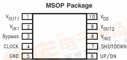
Top View Order Number HWD2111MM
