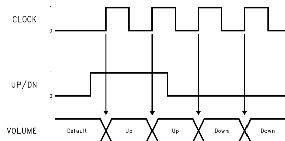
FIGURE 2. Timing Diagram
