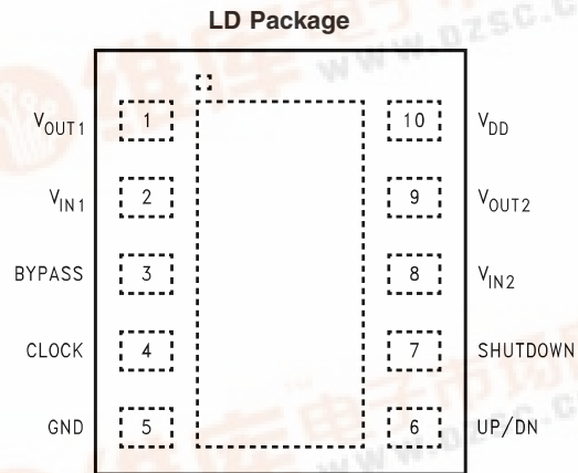
Top View Order Number HWD2111LD
