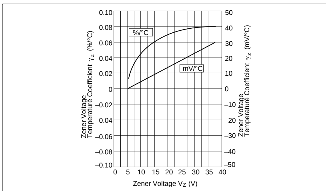
Fig.2 Temperature Coefficient Vs. Zener voltage
