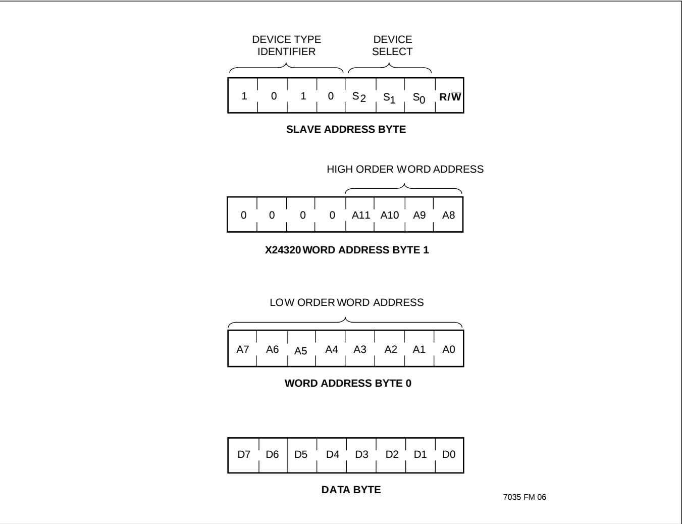
Figure 4. Device Addressing
