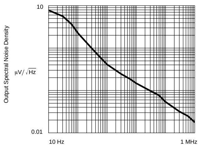
Noise Spectrum
