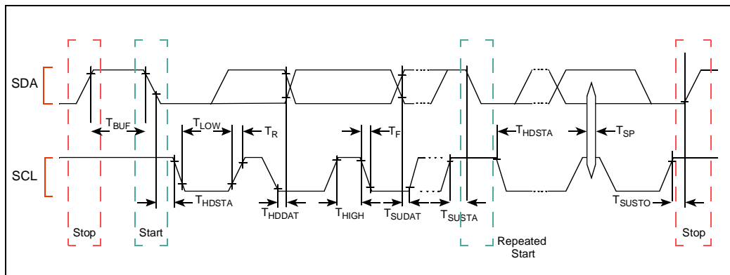
Figure 15. I 2 C Interface Signal Timings
