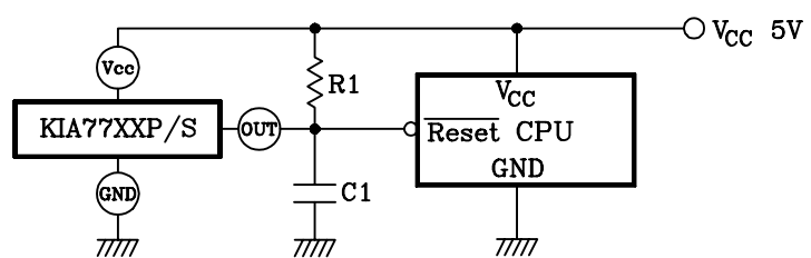
(2) CPU RESETTING
