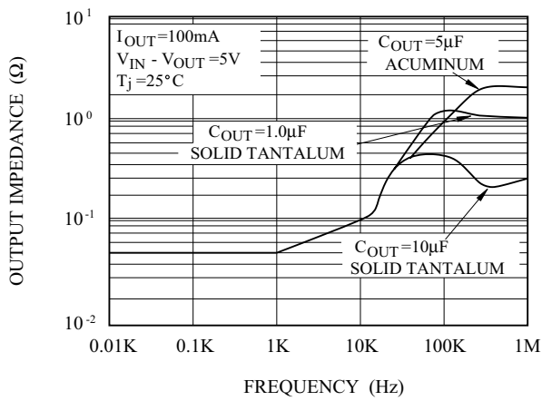
OUTPUT IMPEDANCE
