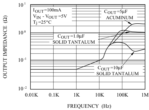
OUTPUT IMPEDANCE
