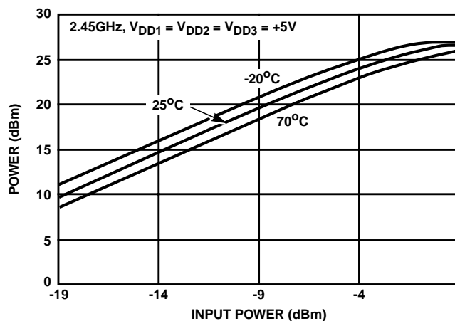
FIGURE 8. POWER OUTPUT
