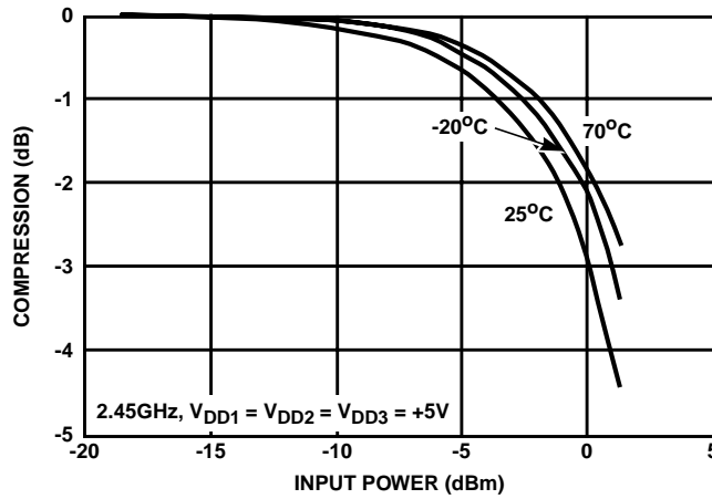
FIGURE 9. GAIN COMPRESSION
