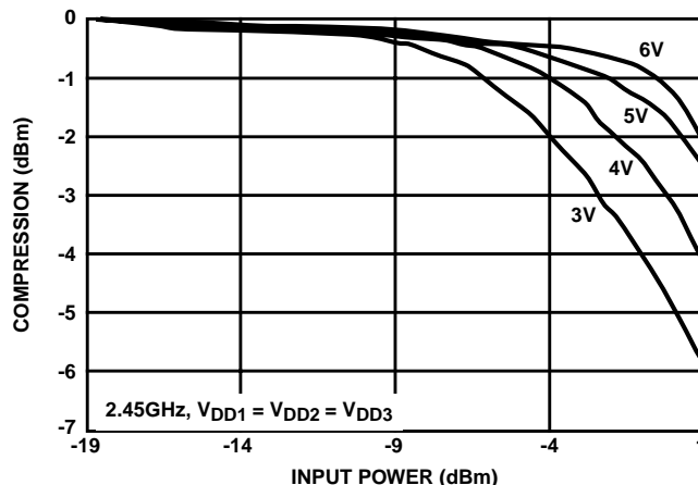
FIGURE 6. GAIN COMPRESSION
