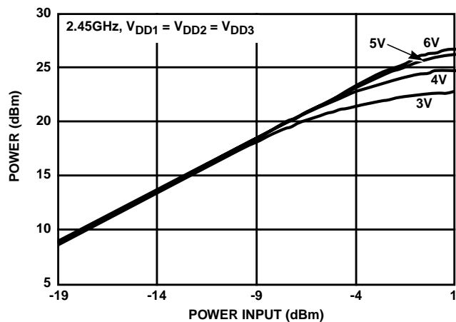
FIGURE 4. POWER OUTPUT
