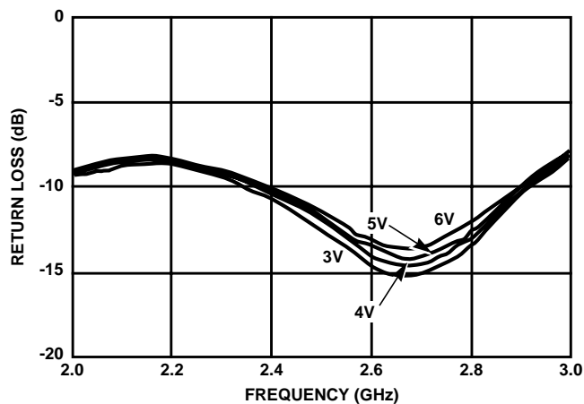
FIGURE 3. OUTPUT MATCH
