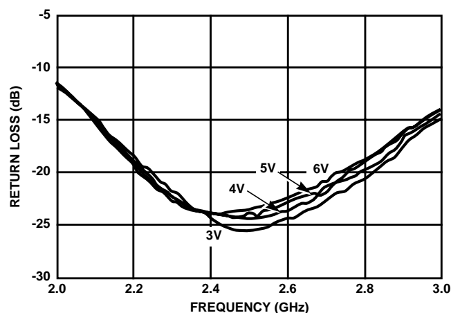
FIGURE 2. INPUT MATCH
