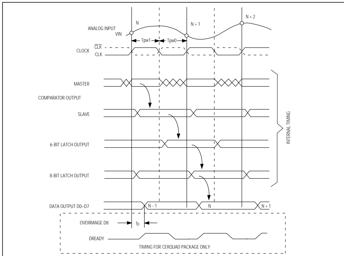
Figure 3. Timing Diagram
