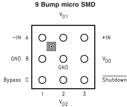
Top View Order Number LM4890IBL, LM4890IBLX See NS Package Number BLA09AAB
