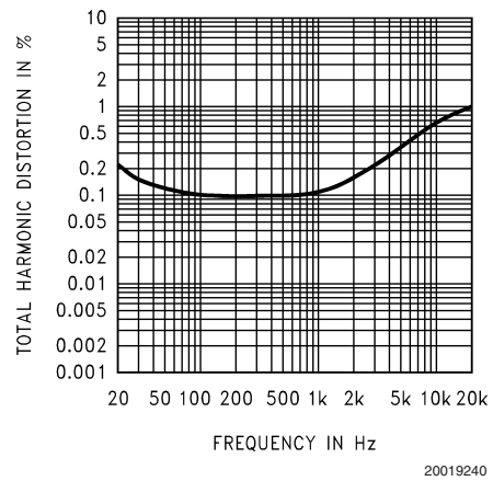
THD+N vs Frequency @ V_{DD} = 2.6V , R_L = 4\Omega , PWR = 100mW , A_V = 2
