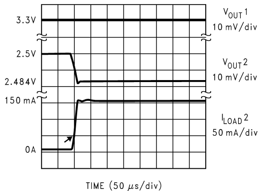
Load Transient Reponse ( V_{OUT2} )
