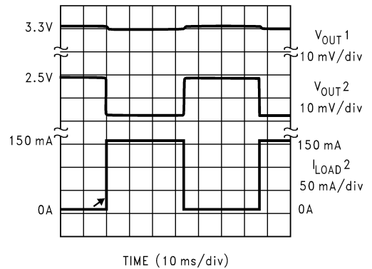
Load Transient Reponse ( V_{OUT2} )
