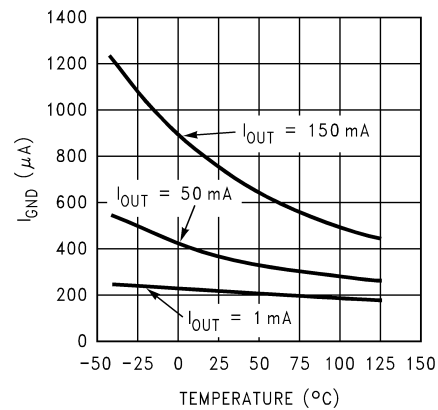
Ground Pin Current vs Temp. and Load
