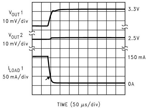
Load Transient Reponse ( V_{OUT1} )
