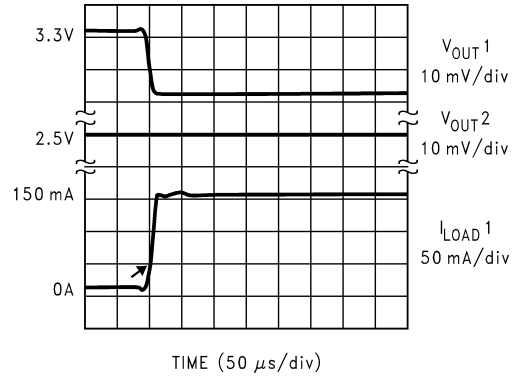
Load Transient Reponse ( V_{OUT1} )
