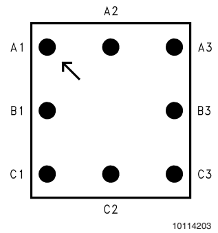
Top View micro SMD 8-Bump micro SMD Package Code: BP
