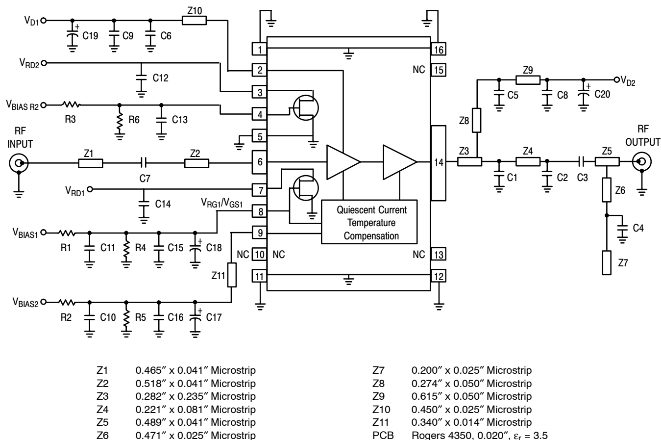
Figure 1. MW5IC2030MBR1(GMBR1) Test Circuit Schematic
