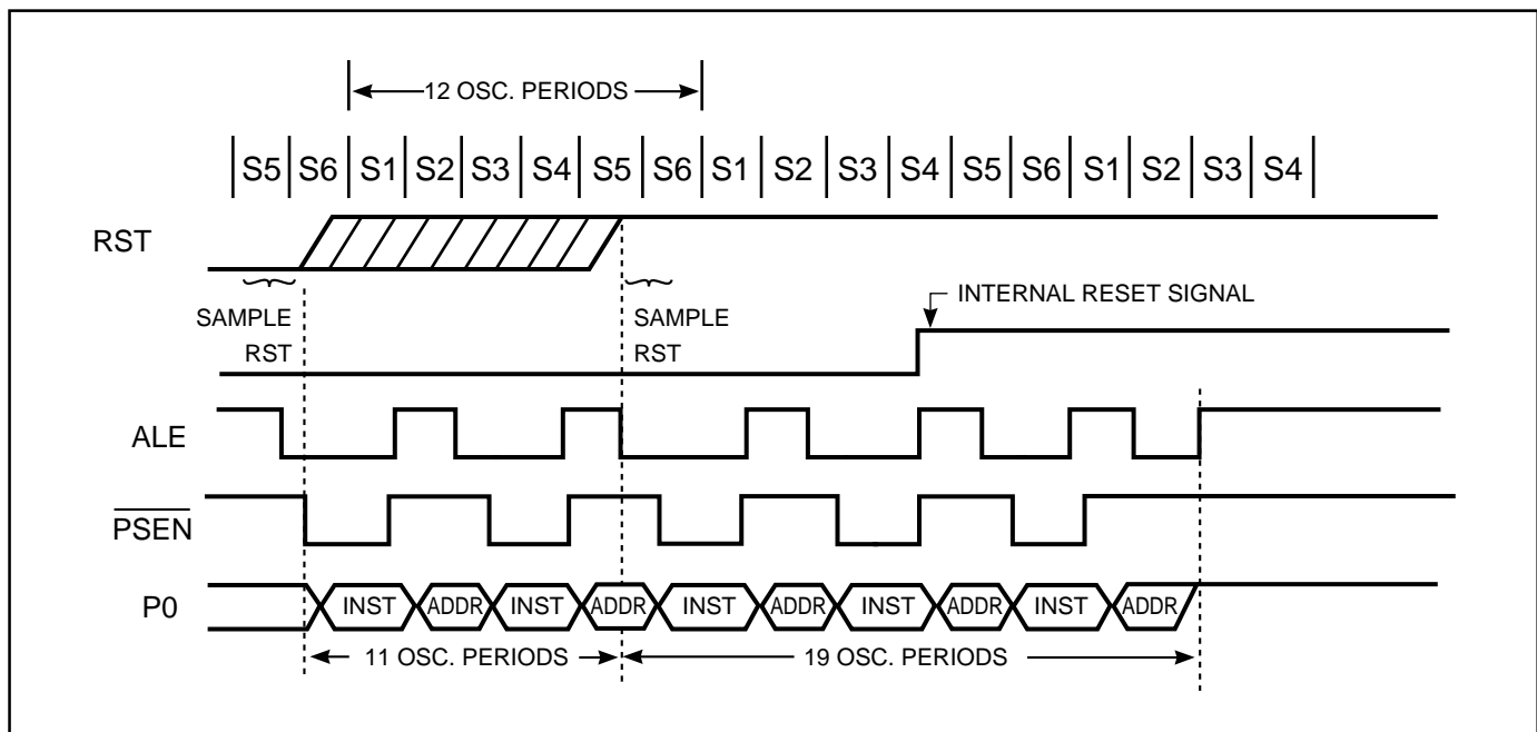
Figure 22. Reset Timing
