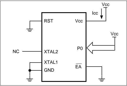
Figure 30. Power-down Mode
