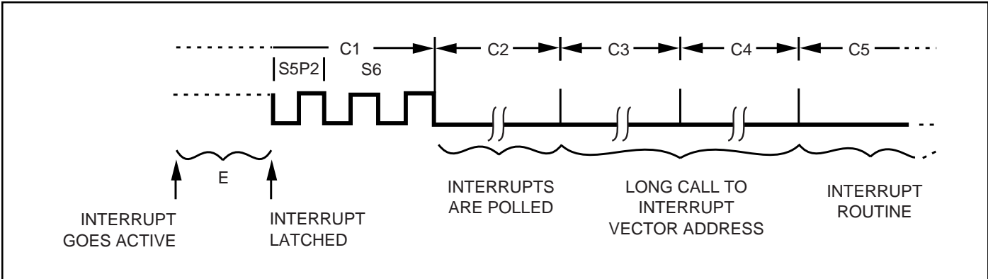
Figure 20. Interrupt Response Timing Diagram
