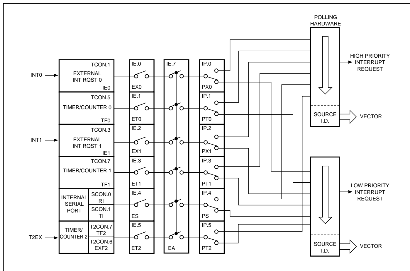
Figure 19. Interrupt System
