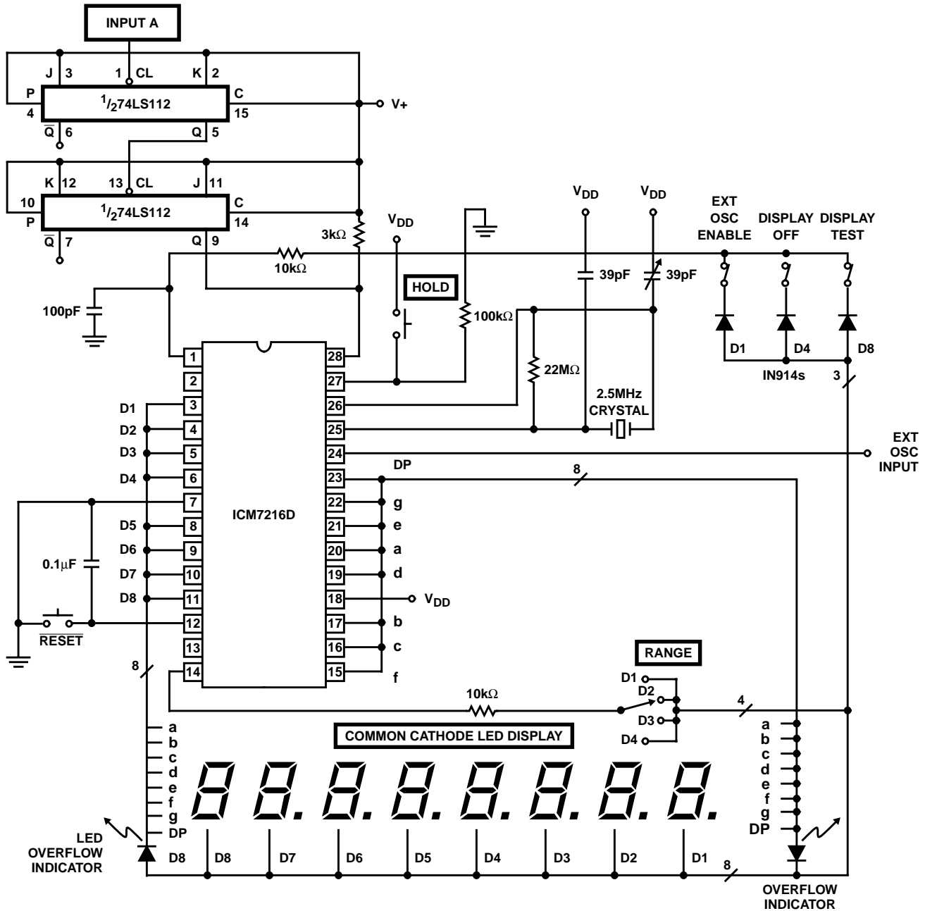
FIGURE 19. 40MHz FREQUENCY COUNTER
