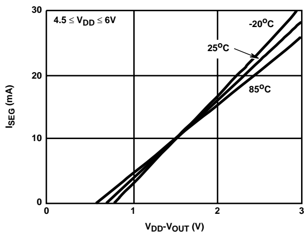
FIGURE 4. ICM7216B AND ICM7216D TYPICAL I_{SEG} vs V_{DD} - V_{OUT}
