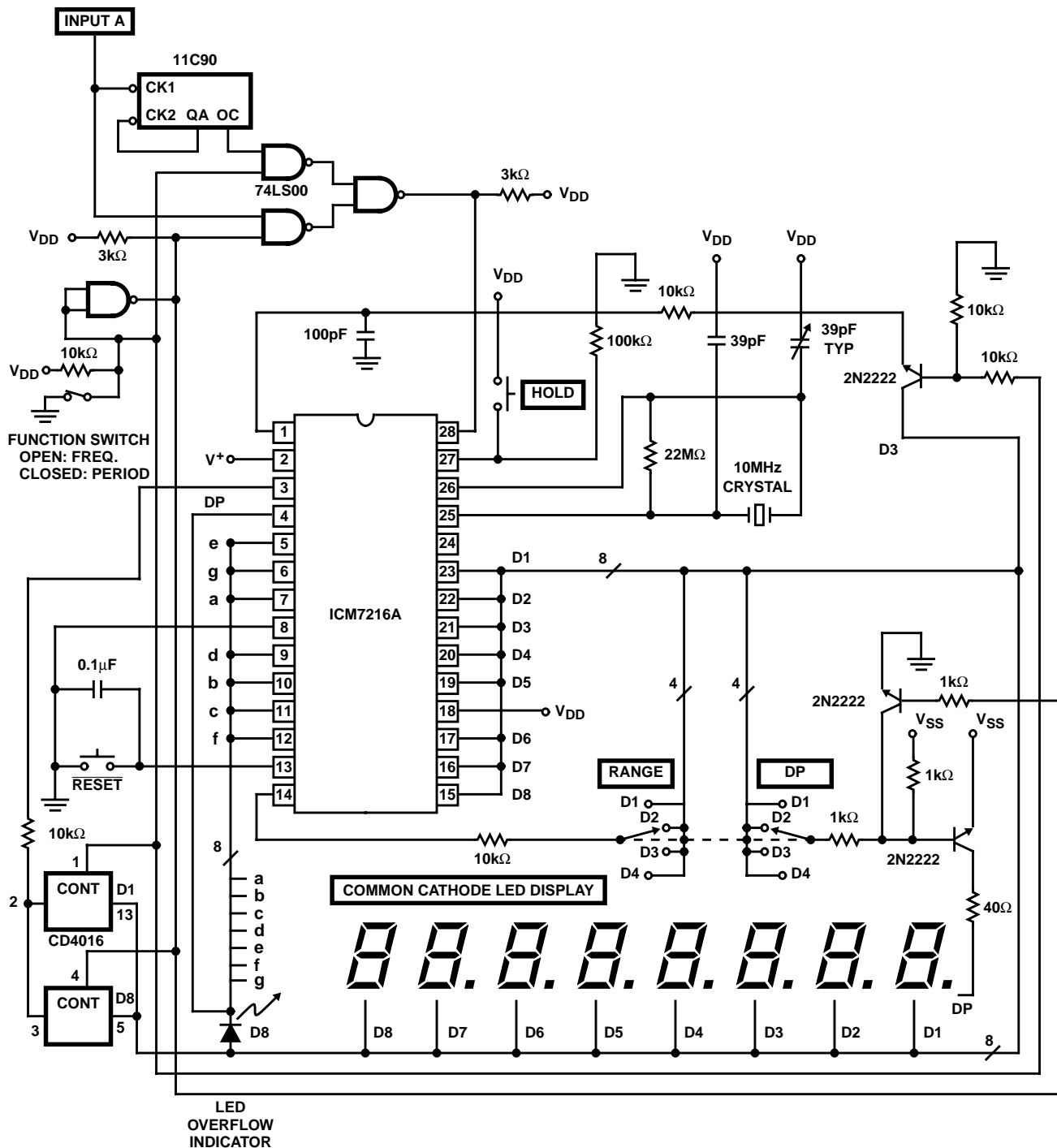
FIGURE 21. 100MHz FREQUENCY, 2MHz PERIOD COUNTER
