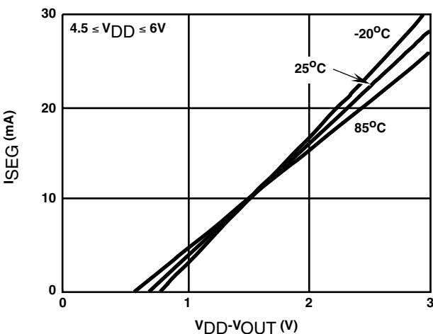
FIGURE 3. TYPICAL I_{SEG} vs V_{DD}-V_{OUT}
