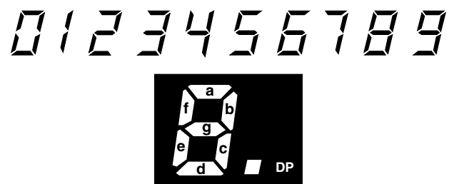
FIGURE 9. SEGMENT IDENTIFICATION AND DISPLAY FONT
