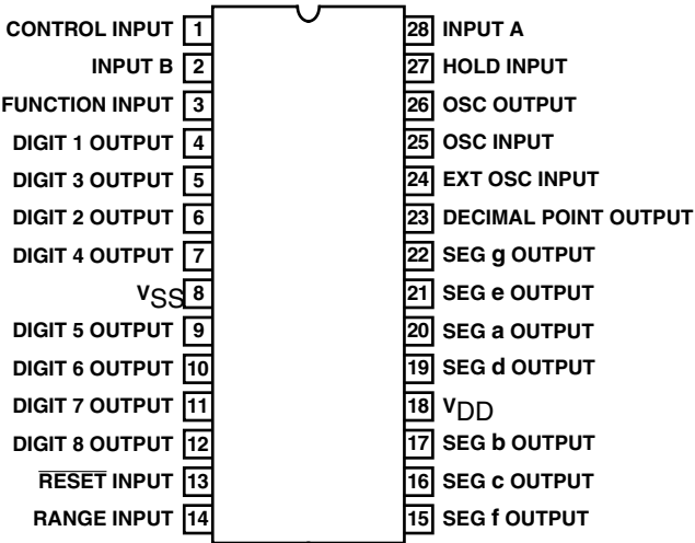
ICM7216D COMMON CATHODE (PDIP) TOP VIEW
