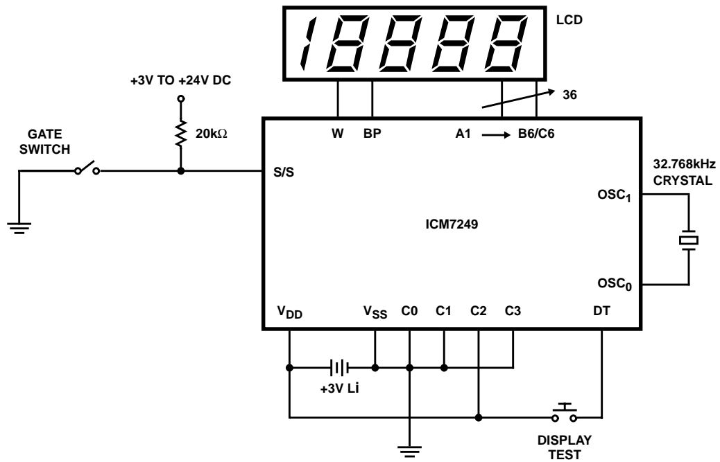
FIGURE 9. ATTENDANCE COUNTER
