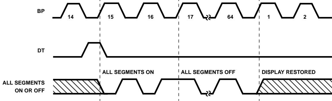
FIGURE 6. DISPLAY TESTING
