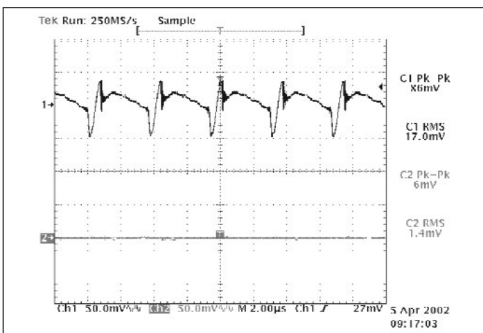
Figure 14 —V48C5C100A and μRAM; Input and output ripple @50% (10A) load CH1=Vi; CH2=Vo; Vi-Vo=327mV; RHR=31k (Configured as in Figs. 1 & 2)
