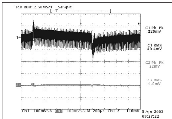
Figure 12 —V300B12C250A and μRAM; Input and output dynamic response no added C TRAN ; 17.5% of 20A rating load step of 3.5A (10A →13.5A);RHR=80k (Configured as in Figs. 1 & 2)
