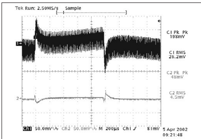
Figure 16 —V48C5C100A and μRAM; Input and output dynamic response C TRAN =820μF Electrolytic; 35% of load step of 7A (10A →17A);RHR=31k (Configured as in Figs. 1 & 2)
