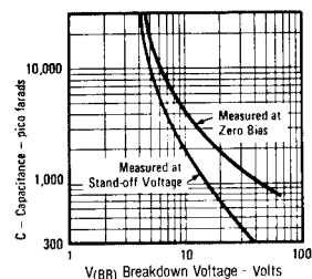
FIGURE 4 TYPICAL CAPACITANCE VS
