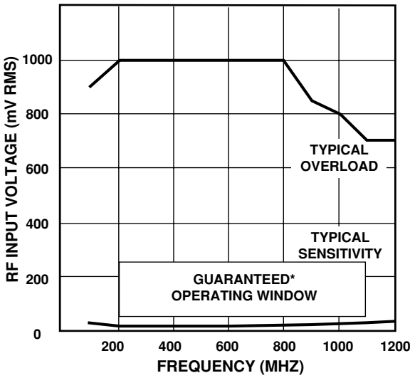
Figure 3 Typical Input Characteristics
