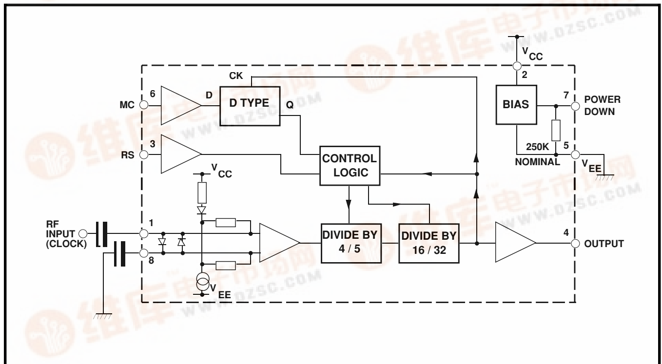
Figure 1 Block Diagram
