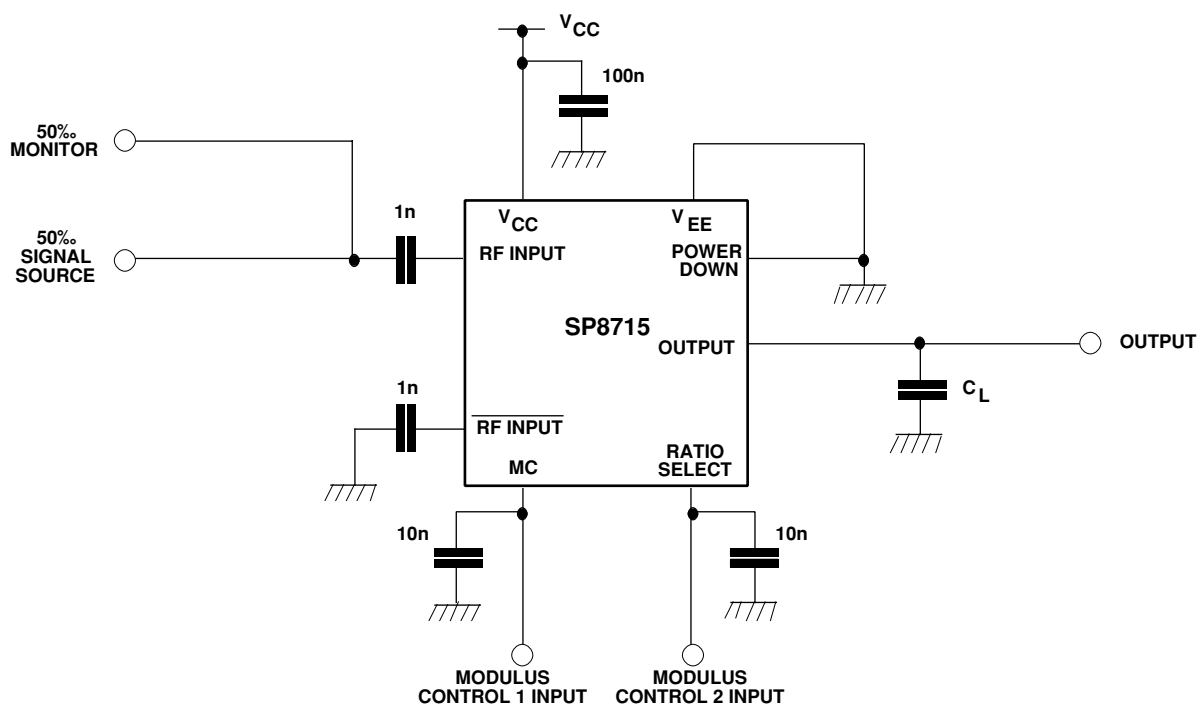
Figure 5 Toggle Frequency Test Circuit
