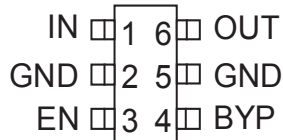
SOT23-6 (Top View)
