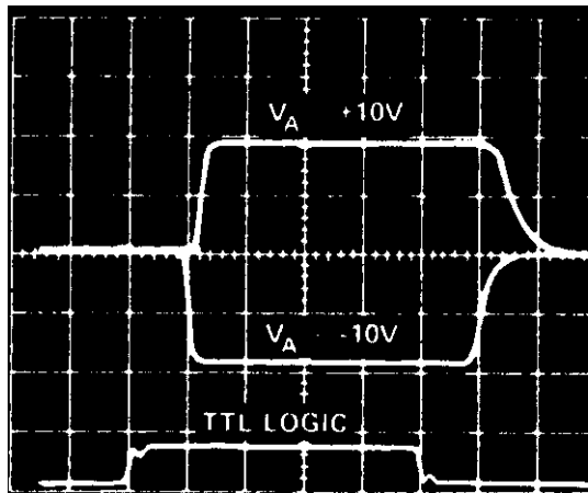
FIGURE 16C. 125°C
