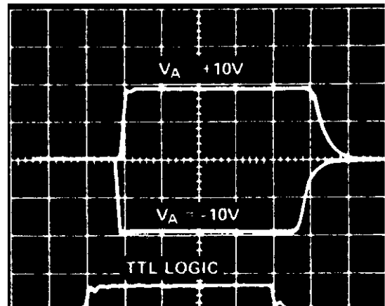
FIGURE 16B. 25°C
