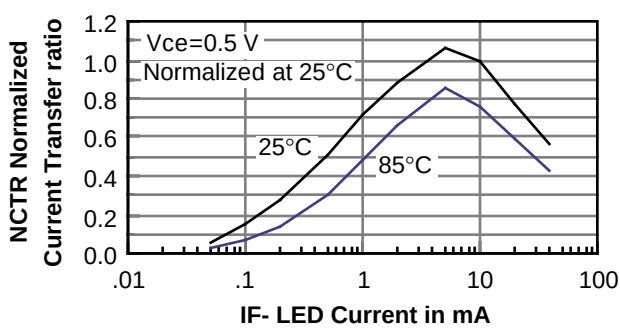
Figure 9. Saturated current transfer ratio, typical
