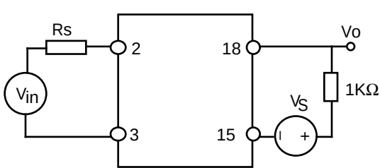
Figure 11. Switching test circuit for SSR channel
