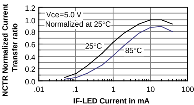
Figure 10. Non-saturated current transfer ratio, typical
