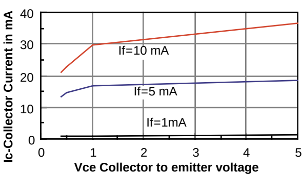
Figure 7. I_C versus V_{CE} , typical
