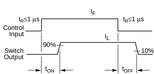
Figure 12. Switching waveform
