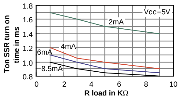
Figure 5. SSR turn on time versus resistive load
