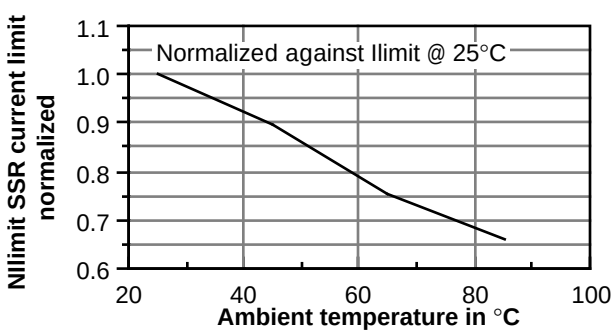
Figure 6. SSR current limit versus temperature
