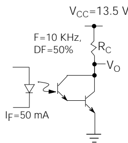
Figure 7. Switching schematic
