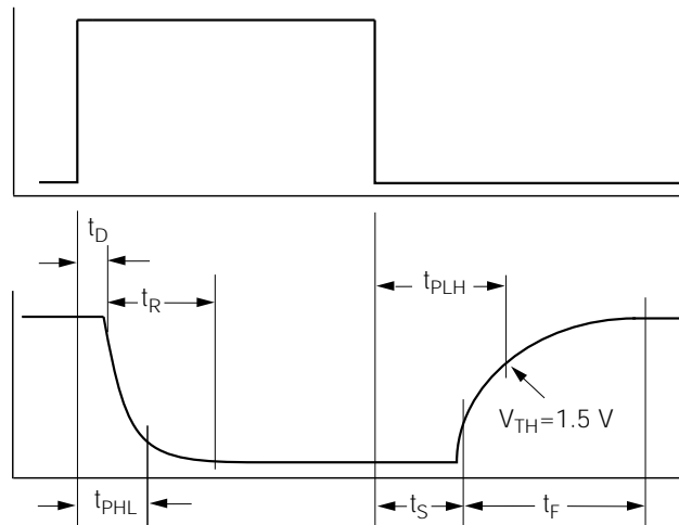
Figure 7. Switching schematic
