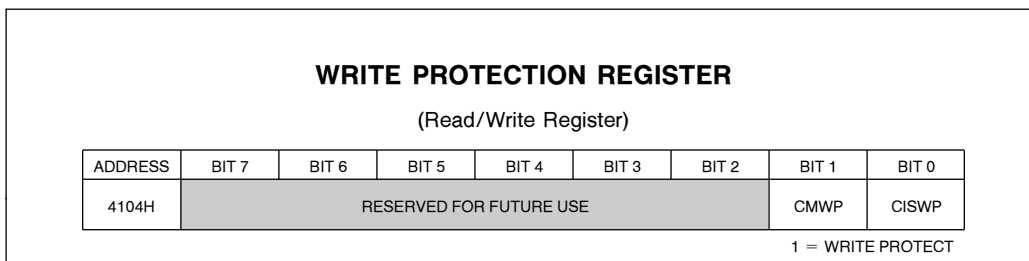
Figure 8. WRITE PROTECTION REGISTER (Intel) Eliminates Accidental Data Corruption
