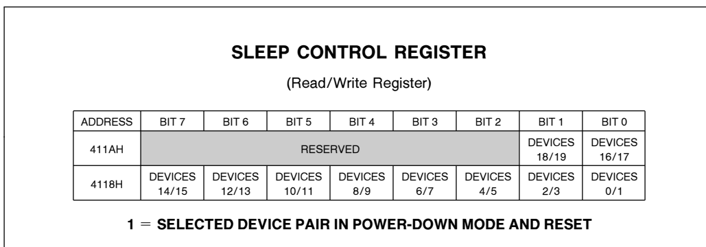
Figure 9. SLEEP CONTROL REGISTER (Intel) Allows Specific Devices to be Reset and Put into Power-Down Mode
