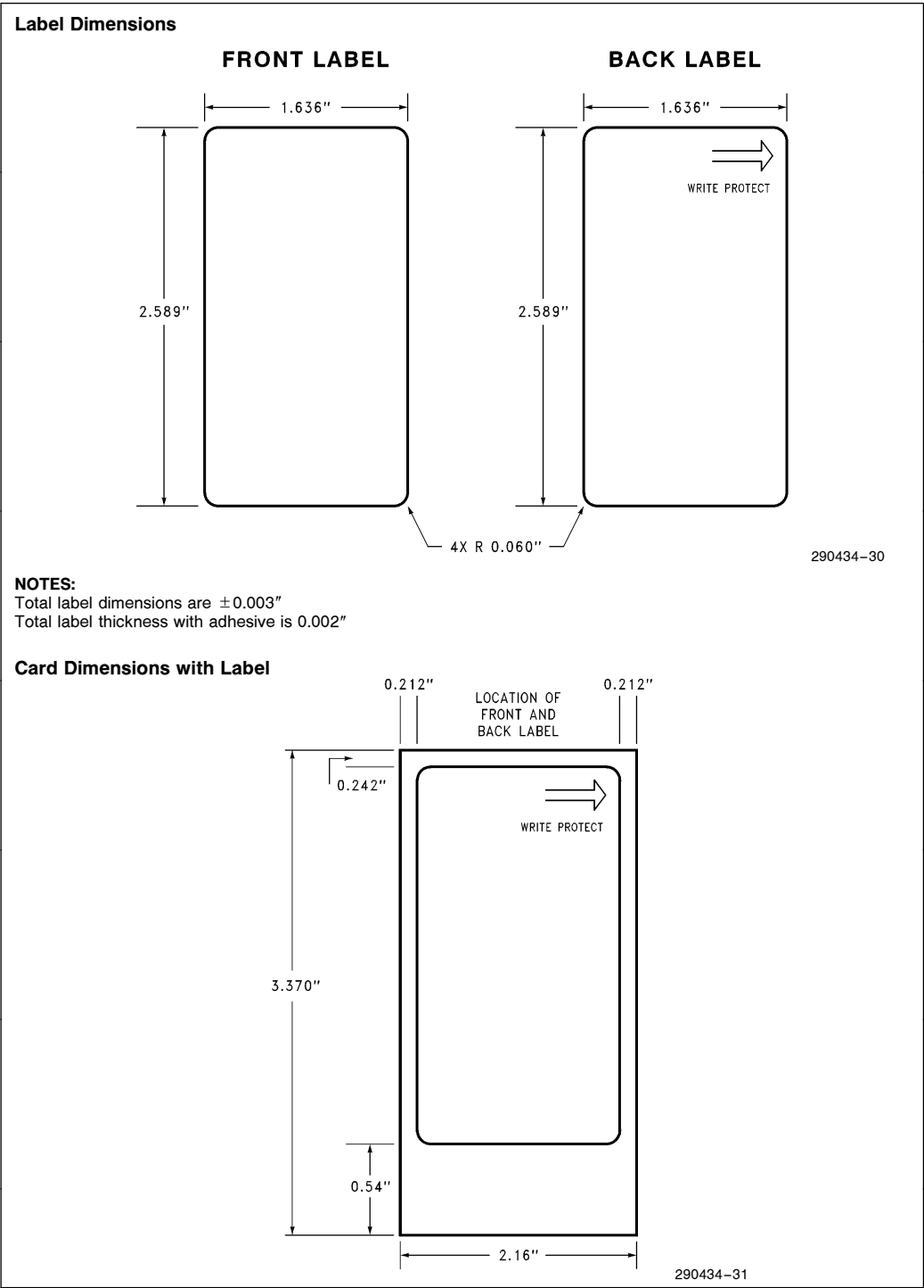
Figure 22. Label Information
