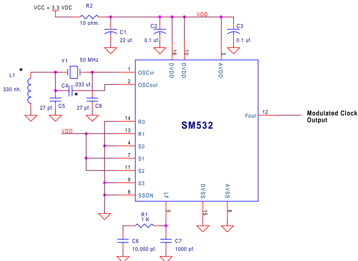
Figure 9. Application Schematic
