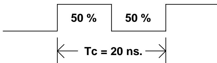
Figure 5. Unmodulated Clock
