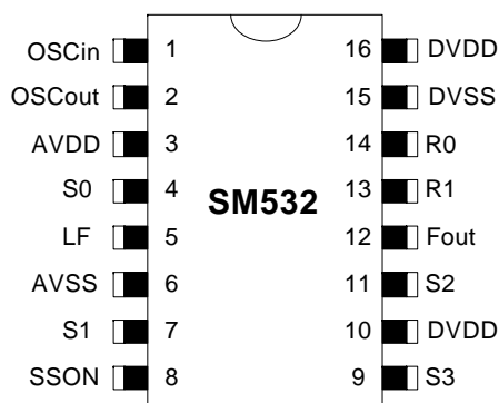
Figure 2. SOIC Package Pin Assignment
