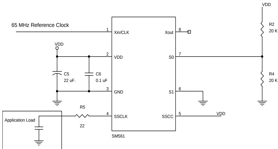
Figure 3. Application Schematic
