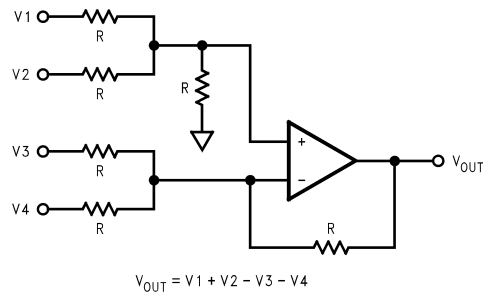
FIGURE 9. Adder/Subtractor Circuit
