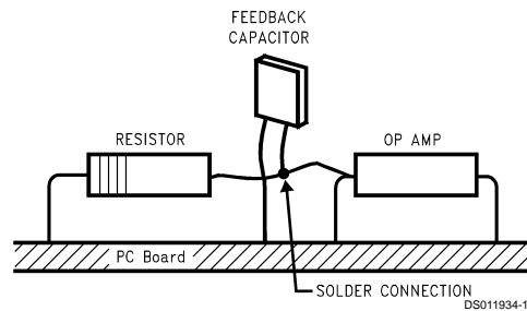
FIGURE 5. Air Wiring
