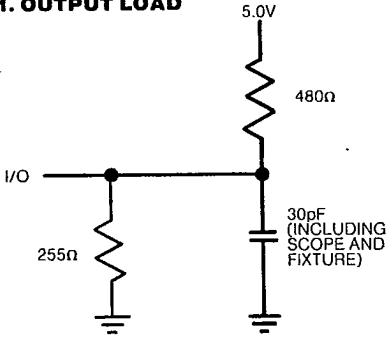
FIGURE 1. OUTPUT LOAD
