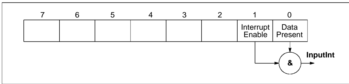
Figure 6.3 IMS C011 Mode 2 input status register
