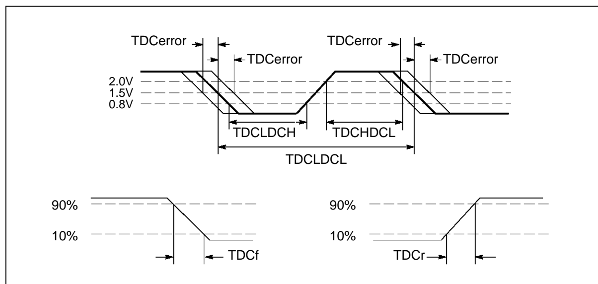
Figure 3.2 ClockIn timing
