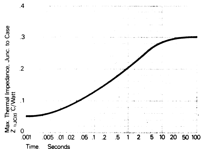
Figure 5. Transient thermal impedance versus time.
