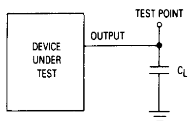
Figure 2. Test Circuit
