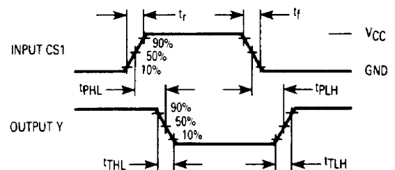
Figure 2. Switching Waveforms
