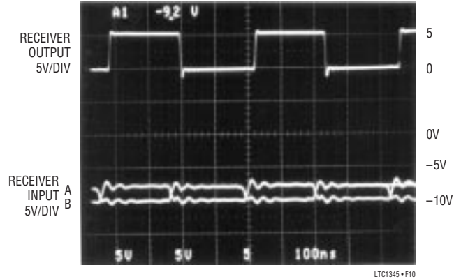
Figure 10. -7V Common Mode
