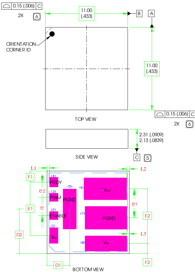
Fig 11: Mechanical Drawing
