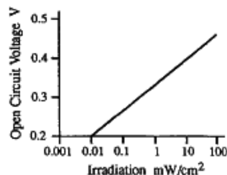
Fig. 3 Open Circuit Voltage
