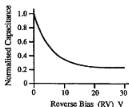
Fig. 2 Normalised Capacitance
