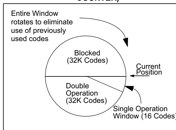
FIGURE 5-3: SYNCHRONIZATION WINDOW (16-BIT COUNTER)
