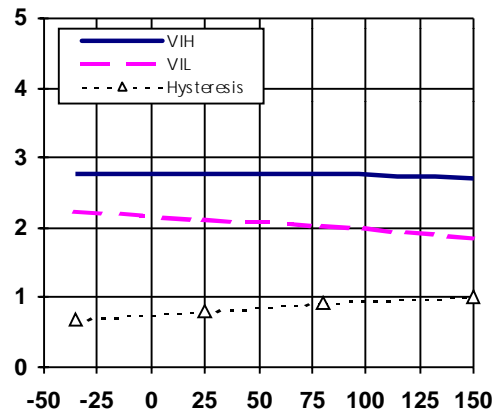
Figure 8 - V IH , V IL threshold ( V ) Vs T j (°C)
