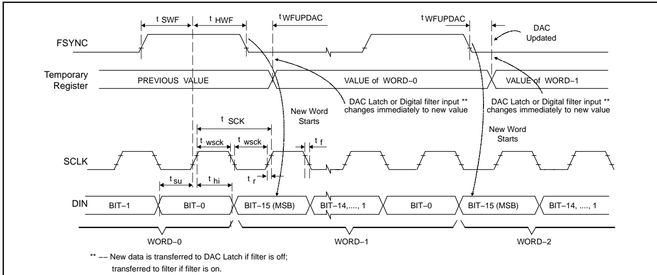
Figure 1. Timing Diagram
