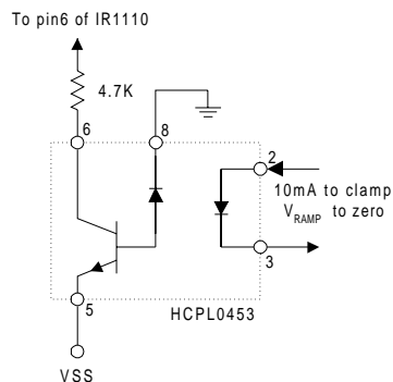
Figure 14 Circuit for Externally Clamping V_{RAMP} to zero
