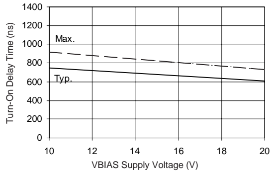
Figure 6B. Turn-On Time vs Voltage
