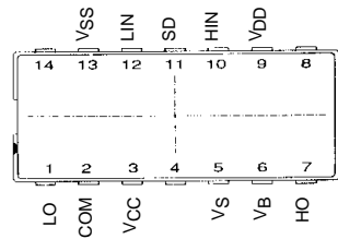
Pin Assignment
