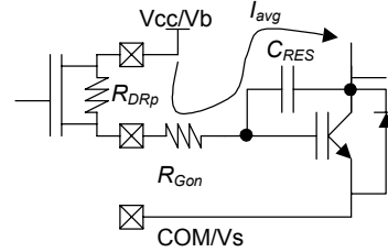
Figure 21: R_{Gon} sizing
