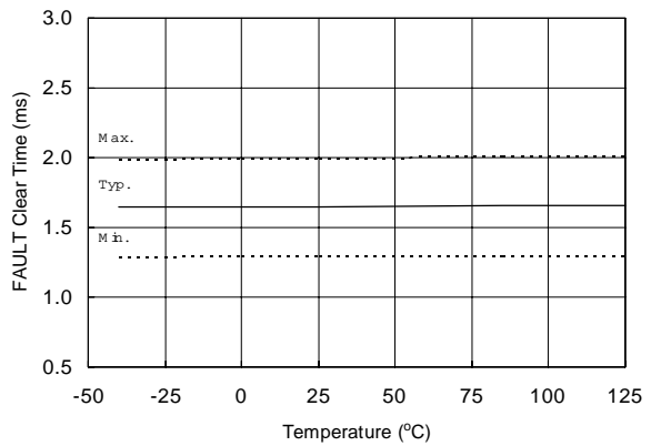
Figure 13A. FAULT Clear Time vs. Temperature
