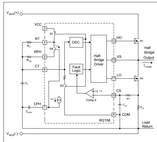
Figure 4, Ignition circuitry.
