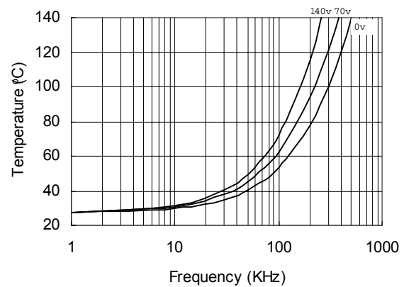
Figure 36. IR21814s vs. Frequency (IRFPE50), R_{gate} = 10\Omega, V_{CC} = 15V
