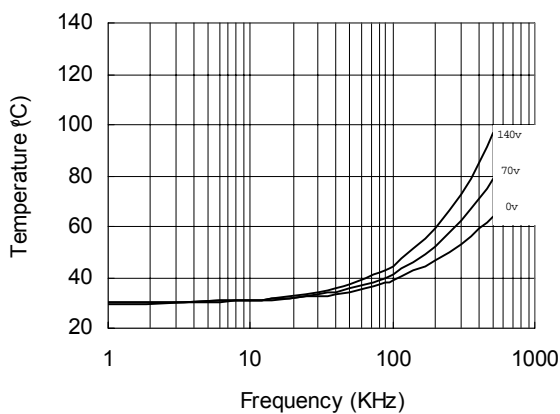
Figure 35. IR21814s vs. Frequency (IRFBC 40), R_{gate} = 15\Omega, V_{CC} = 15V
