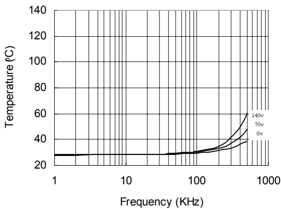
Figure 33. IR21814s vs. Frequency (IRFBC 20), R_{gate} = 33\Omega, V_{CC} = 15V
