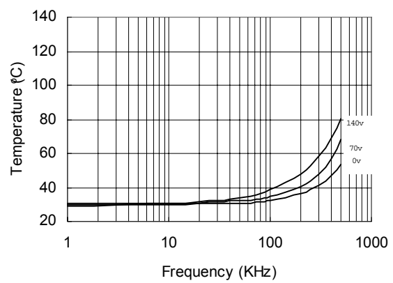
Figure 34. IR21814s vs. Frequency (IRFBC 30), R_{gate} = 22\Omega, V_{CC} = 15V
